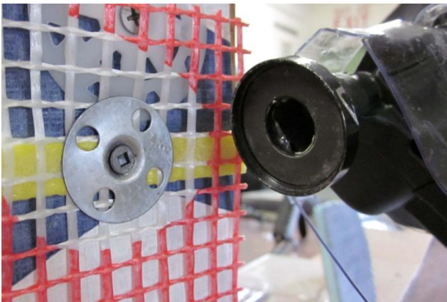
1¼" dia. Grip-Plate® on Spider Lath
